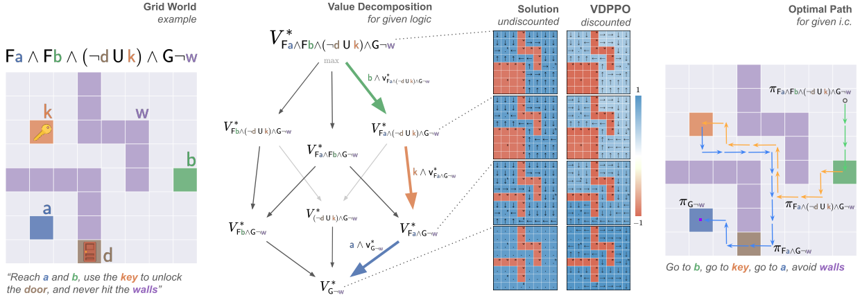
Fig. 2: N-AND-Until Value Decomposition . Here we illustrate the primary decomposition result (Thm. 2 extension, Appendix), with a GridWorld example (left) for a given specification. The corresponding DVG is shown (center left) with each node representing a decomposed Value, and edges representing dependencies. In the center right, a subset of decomposed Values solved with dynamic programming are shown, along with the discounted solution produced by VDPPO. On the right, the optimal path for a given initial condition is shown.
