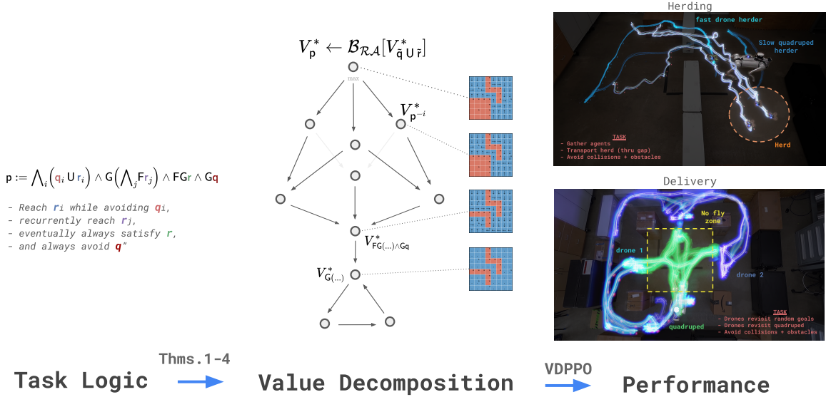
Fig. 1: Value-Decomposition and VDPPPO. The Bellman Value for a range of temporal logic (e.g., multi-goal, recurrence, stability, safety) decomposes into a Value graph connected by atomic Bellman equations (Thms. 1–4). We propose VDPPPO, an algorithm that exploits this structure to learn policies for complex, high-dimensional tasks. Our approach is validated on hardware with Herding and Delivery, two complex tasks involving a heterogeneous team of drones and a quadruped.
