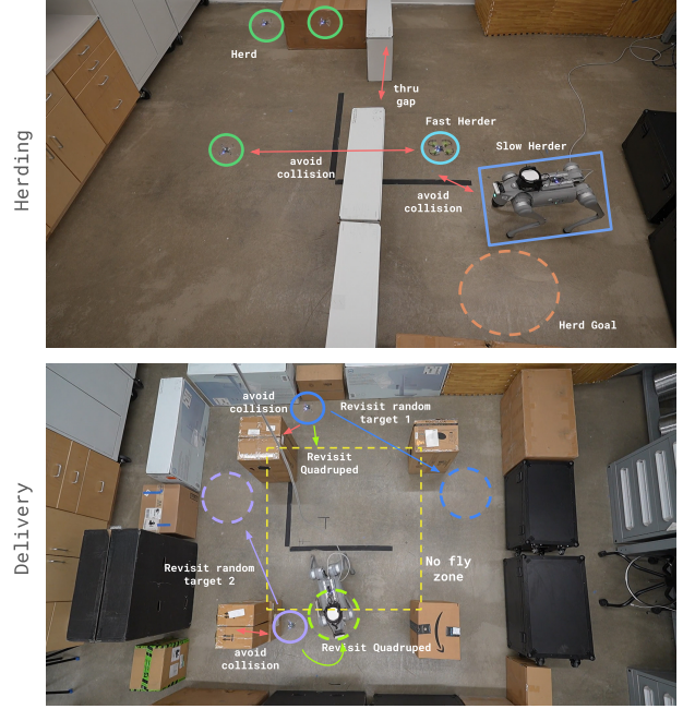
Fig. 7: Hardware Overview for Herding and Delivery Tasks
