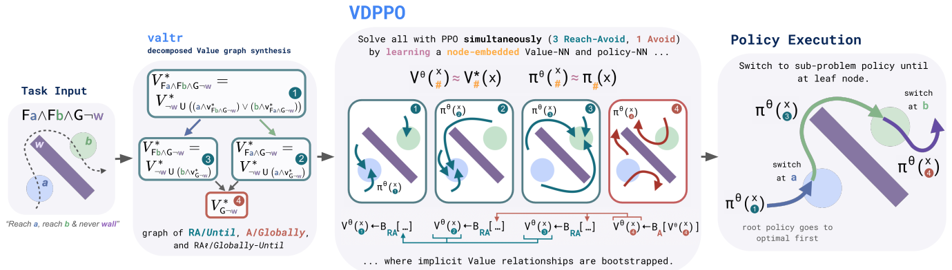
Fig. 4: Graphical Depiction of valtr and VDPPO.
